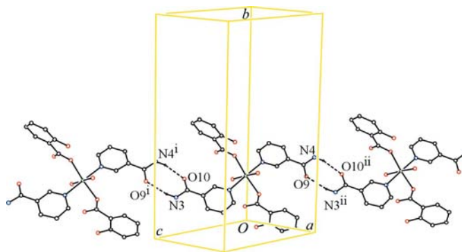
Figure 3 Part of the crystal structure of (I), showing the formation of an R_2^2(8) dimer. Hydrogen bonds are indicated by dashed lines. H atoms not involved in these interactions have been omitted for clarity. (Symmetry codes as in Table 2.)
