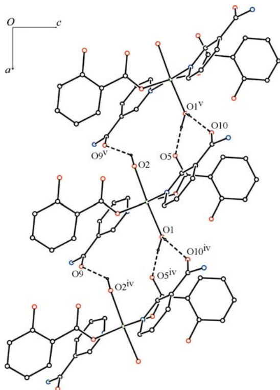
Figure 2 Part of the crystal structure of (I), showing the formation of R_2^2(12) and R_2^2(14) rings. Hydrogen bonds are indicated by dashed lines. H atoms not involved in these interactions have been omitted for clarity. (Symmetry codes as in Table 2.)
