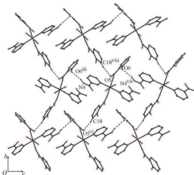
Figure 4 Part of the crystal structure of (I), showing the formation of a chain of edge-fused R_4^4(40) rings. Hydrogen bonds are indicated by dashed lines. For the sake of clarity, H atoms not involved in the motif shown have been omitted. [Symmetry codes: (iii) x, y, z - 1 ; (vi) -x, y - \frac{1}{2}, -z ; (vii) x, y, z + 1 ; (viii) -x, y + \frac{1}{2}, -z .]
